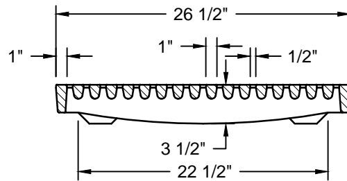
GRATE SECTION B-B
