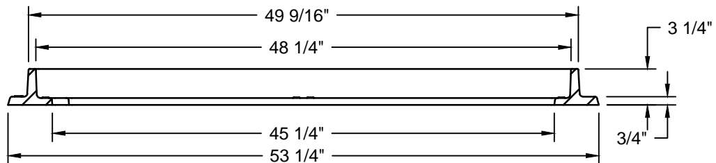
FRAME SECTION A-A
