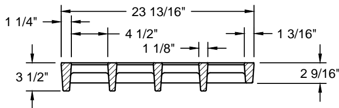
GRATE SECTION A-A
