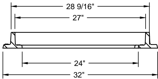
FRAME SECTION B-B
