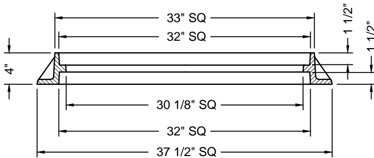
FRAME SECTION
