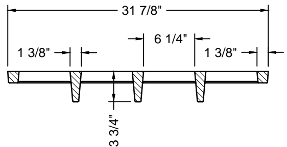
GRATE SECTION B-B
