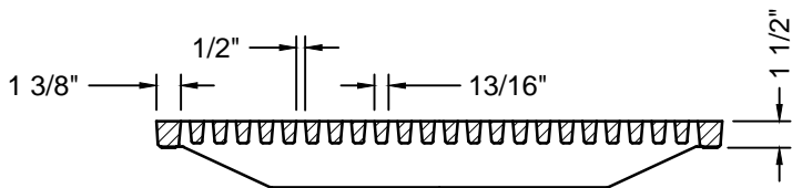
FRAME SECTION
