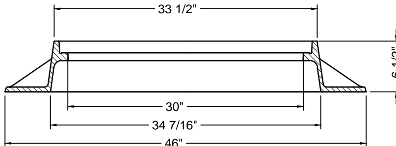
FRAME SECTION
