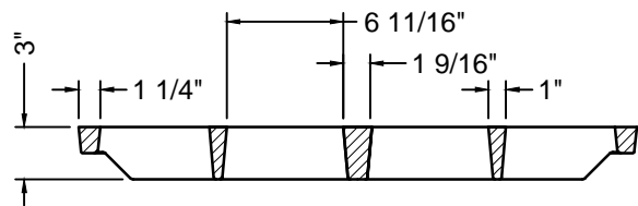
GRATE SECTION B-B
