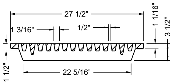
GRATE SECTION A-A
