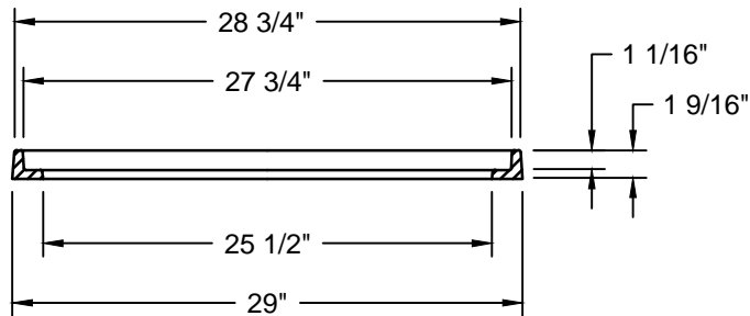
FRAME SECTION
