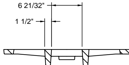
GRATE SECTION B-B
