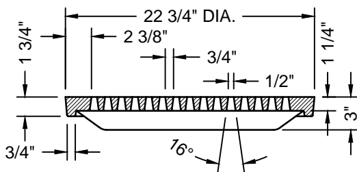
GRATE SECTION A-A
