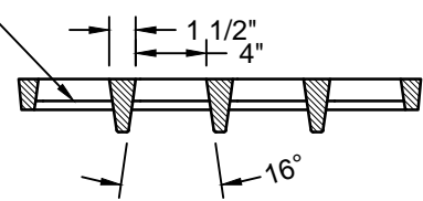
GRATE SECTION B-B
