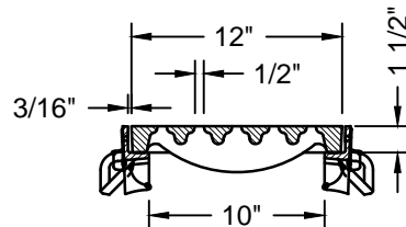
TYPICAL SECTION
