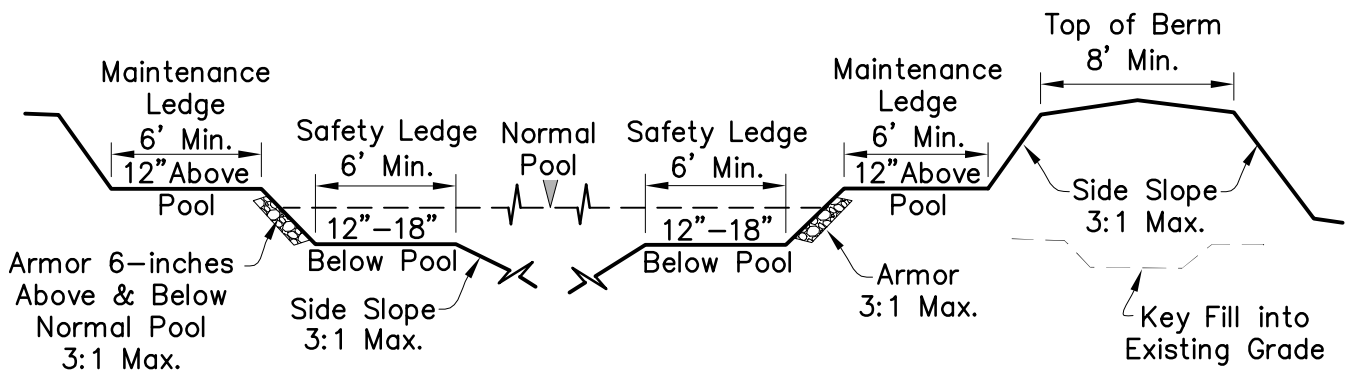
Cross-Section B-B
