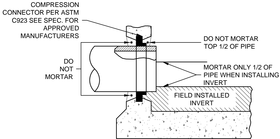
COMPRESSION TYPE CAST IN PLACE
