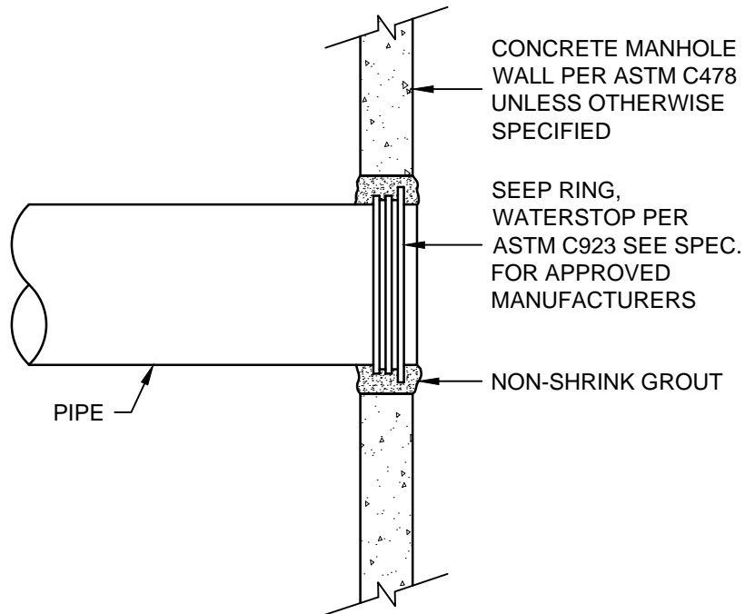
COMPRESSION TYPE GROUT IN PLACE
