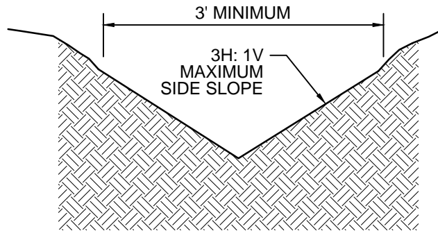
TYPICAL GRASS LINED DITCH
