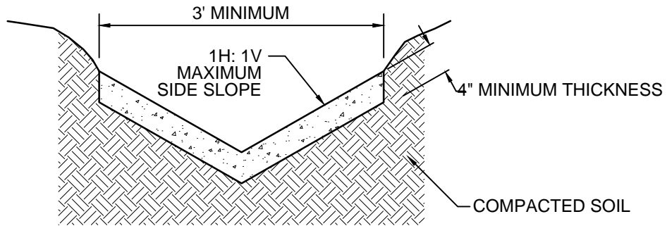
TYPICAL CONCRETE LINED DITCH
