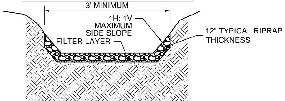
TYPICAL RIPRAP CHANNEL
