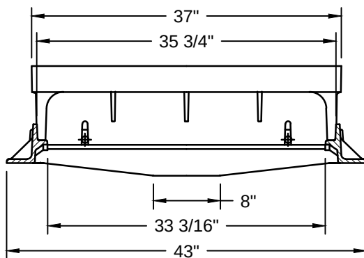
GRATE SECTION C-C
