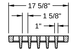
GRATE SECTION B-B
