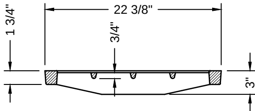
GRATE SECTION C-C
