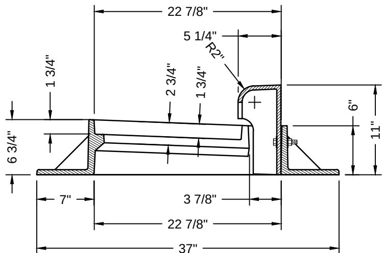
FRAME SECTION B-B
