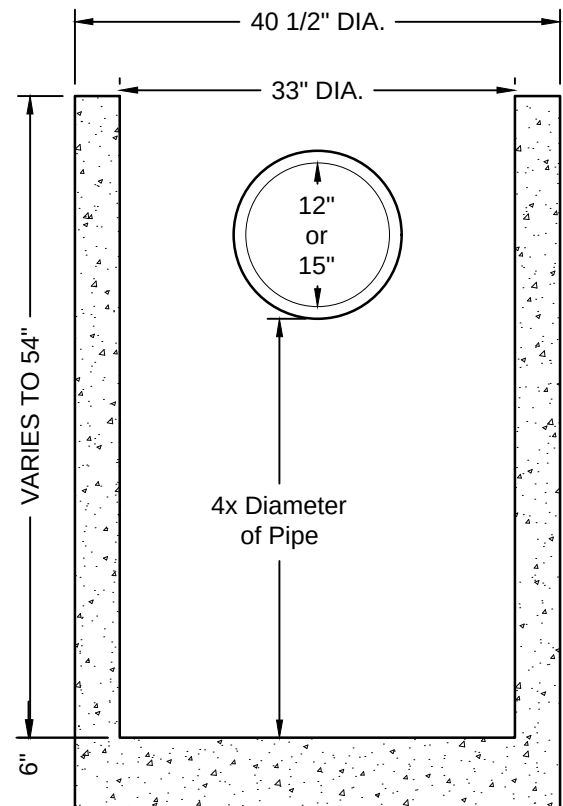
SECTION VIEW B-B
