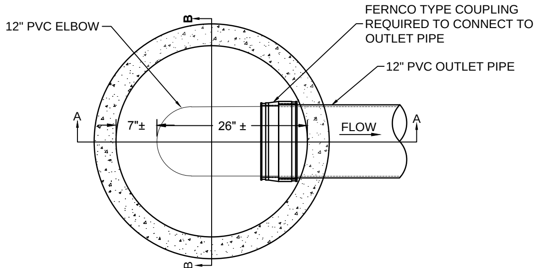
PLAN VIEW
