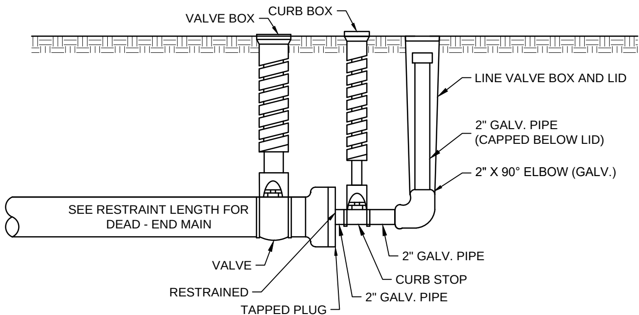
PERMANENT BLOW-OFF ASSEMBLY INSTALLATION
