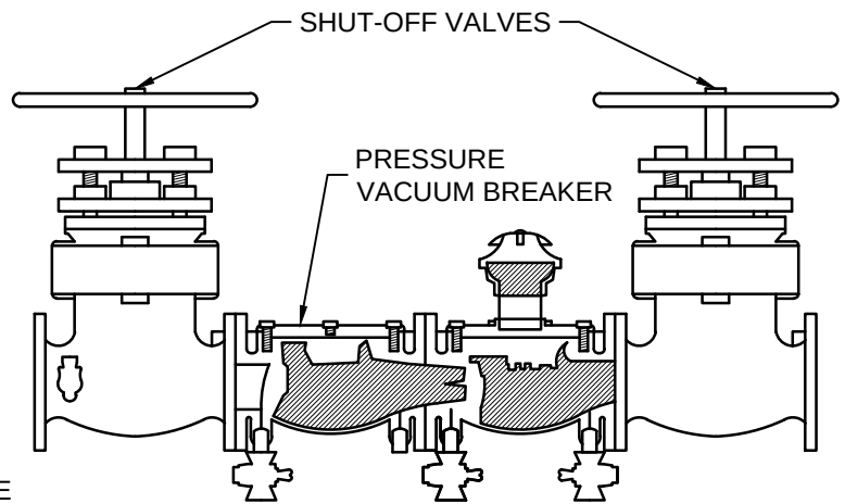
PRESSURE VACUUM BREAKER 2 1/2" TO 10"
