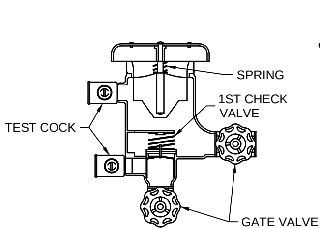
PRESSURE VACUUM BREAKER 3/4" TO 2"
