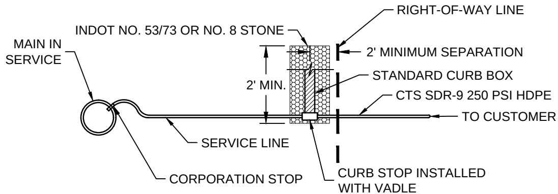
SMALL SERVICE INSTALLATION 3/4" THRU 2" (MIN. 5' COVER)
