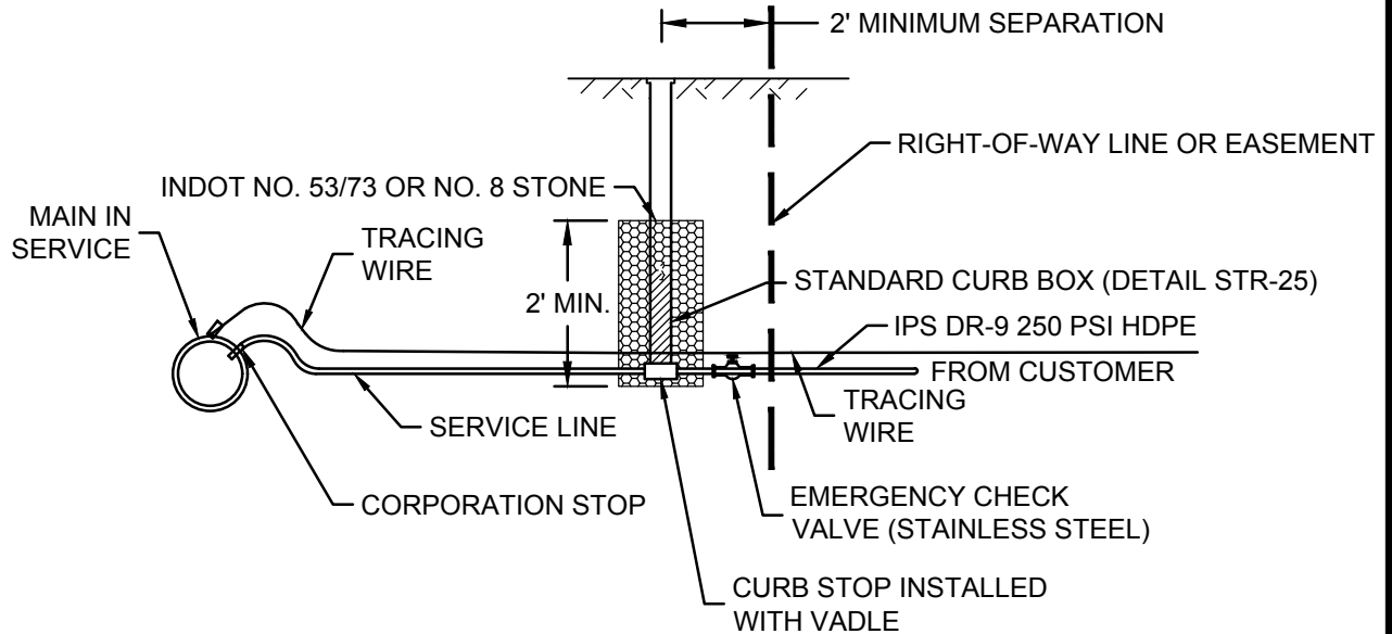
SMALL SERVICE INSTALLATION 1.5" THRU 2" (MIN. 5' COVER)
